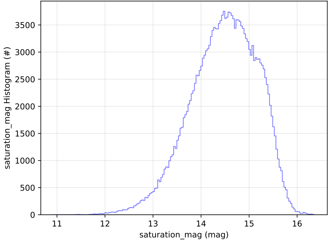
too_elab_2yr_r64_d3_ugrizy_v3.4_10yrs All sky g band: saturation_mag Histogram
