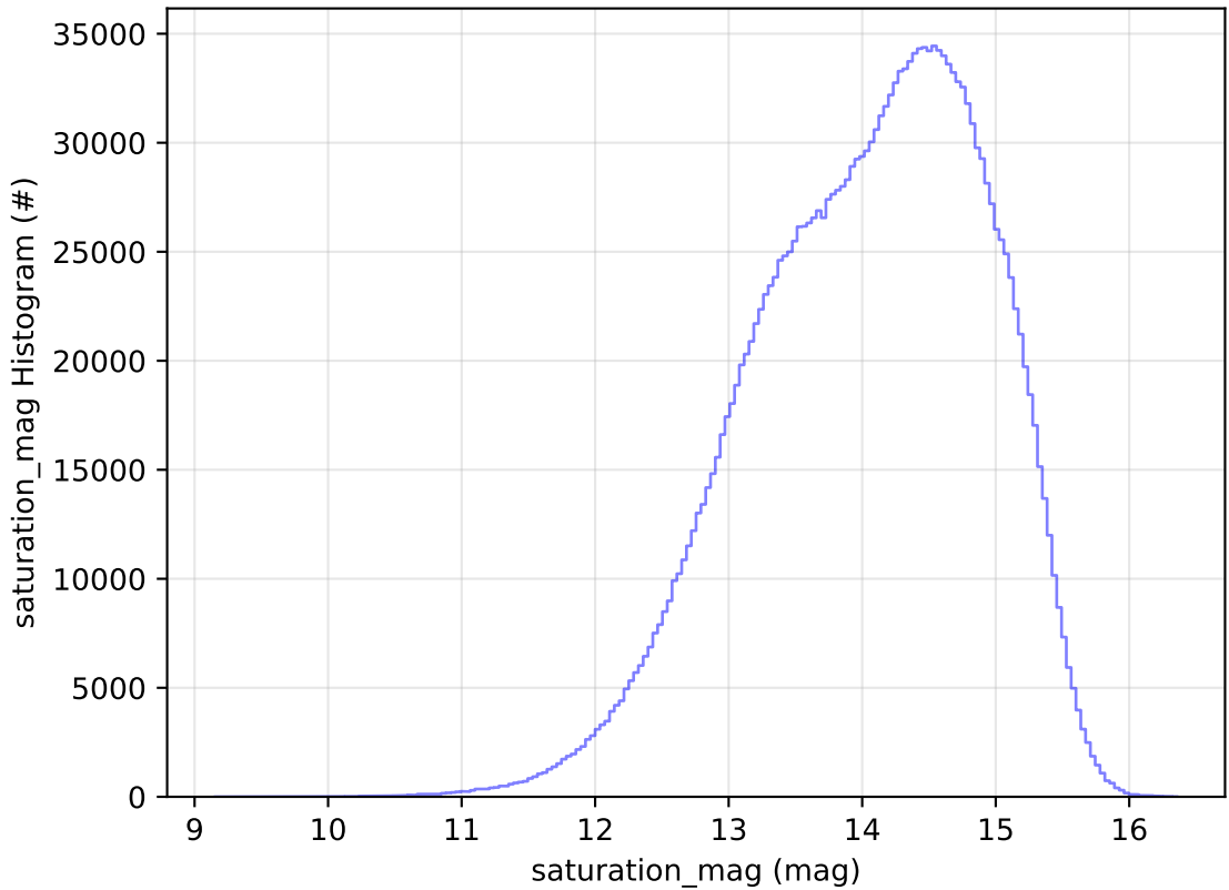
too_elab_2yr_r64_d3_ugrizy_v3.4_10yrs All sky all bands: saturation_mag Histogram
