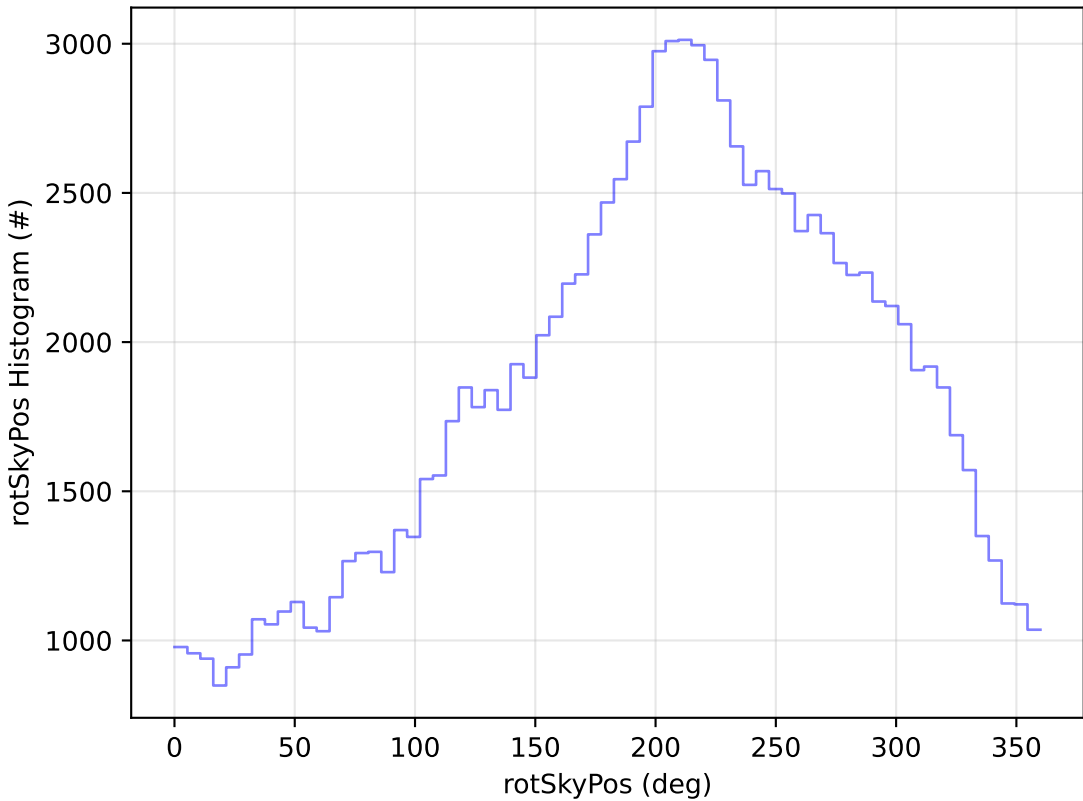
too_elab_2yr_r64_d3_ugrizy_v3.4_10yrs WFD u band: rotSkyPos Histogram
