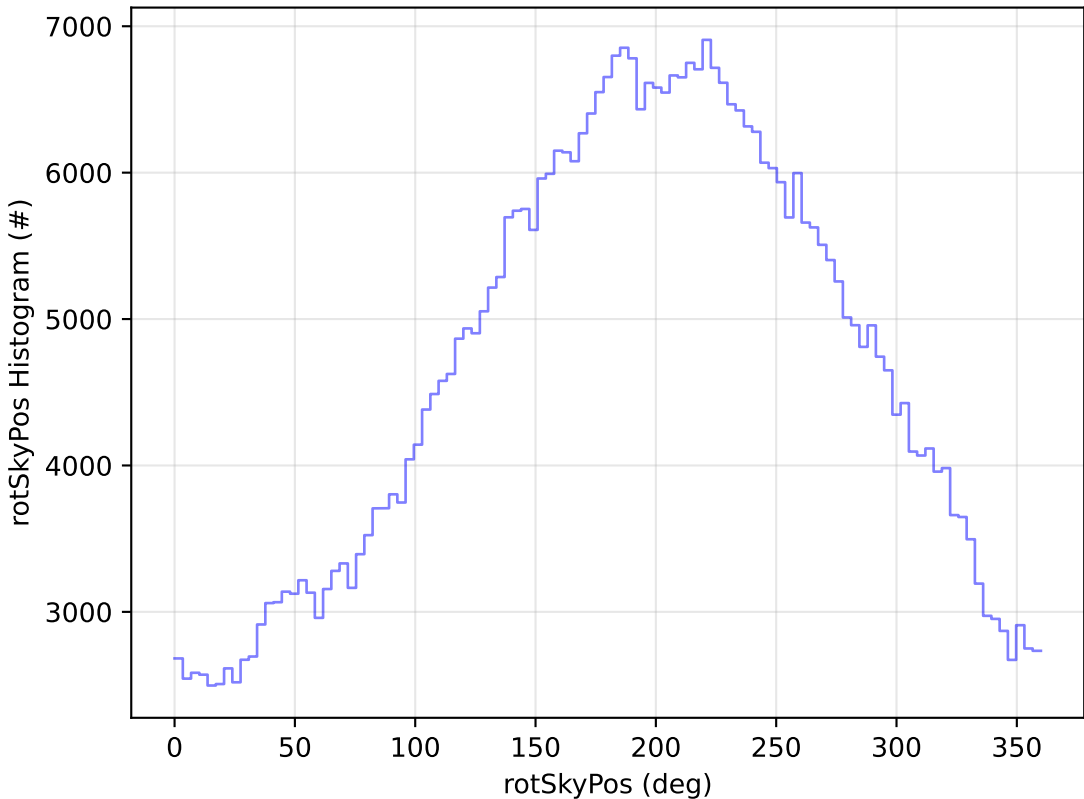
too_elab_2yr_r64_d3_ugrizy_v3.4_10yrs WFD r band: rotSkyPos Histogram
