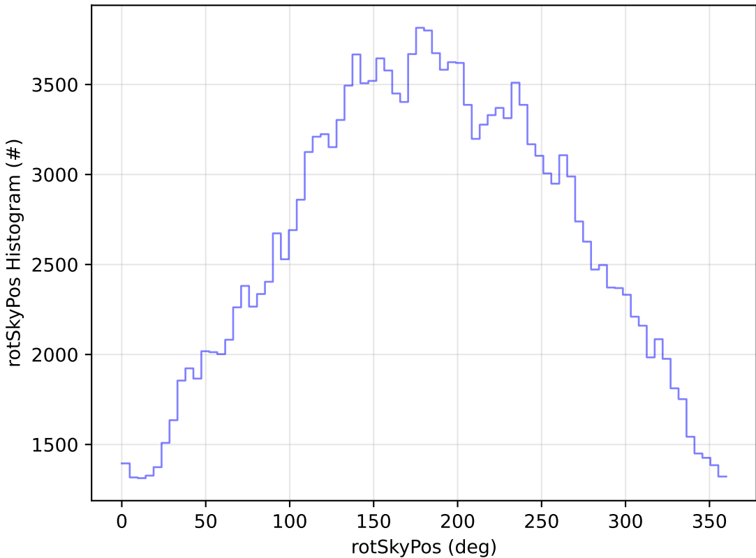
too_elab_2yr_r64_d3_ugrizy_v3.4_10yrs WFD g band: rotSkyPos Histogram
