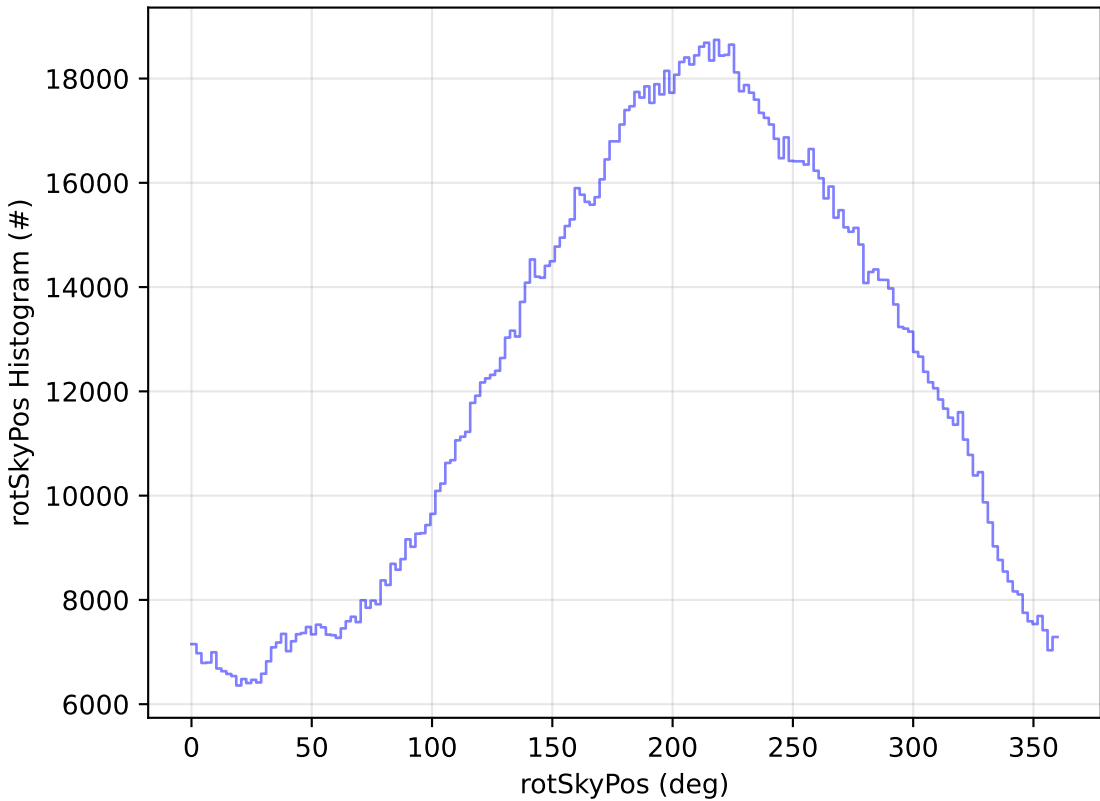
too_elab_2yr_r64_d3_ugrizy_v3.4_10yrs WFD all bands: rotSkyPos Histogram
