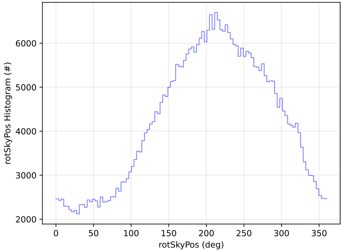
too_elab_2yr_r64_d3_ugrizy_v3.4_10yrs All sky z band: rotSkyPos Histogram
