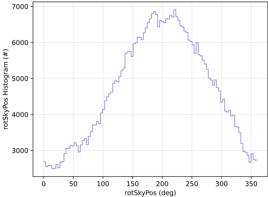
too_elab_2yr_r64_d3_ugrizy_v3.4_10yrs All sky r band: rotSkyPos Histogram
