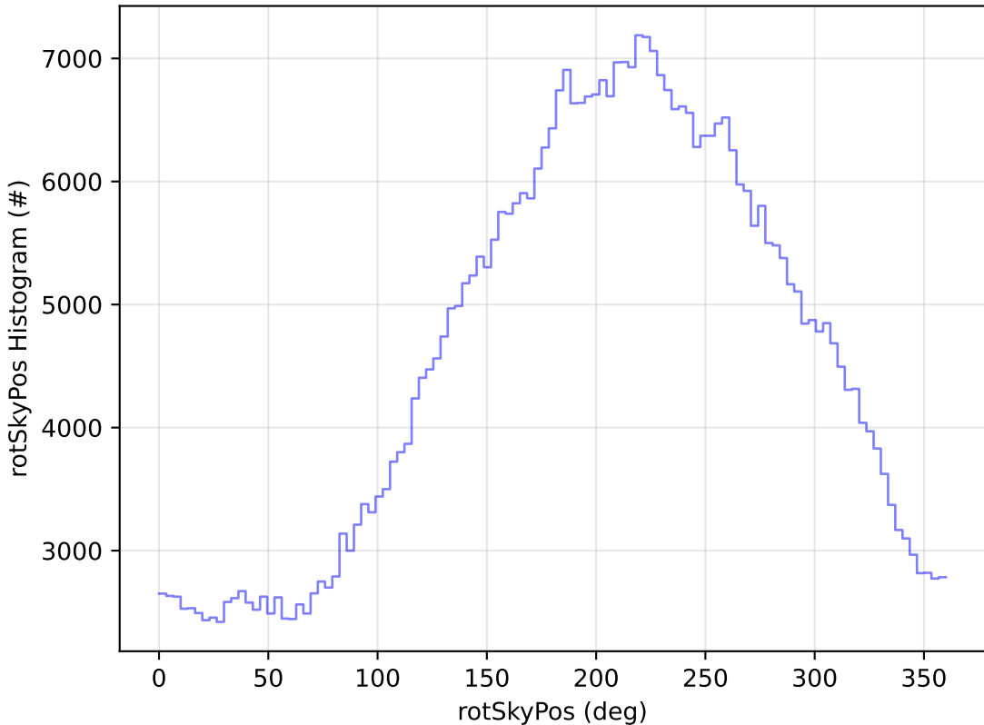
too_elab_2yr_r64_d3_ugrizy_v3.4_10yrs All sky i band: rotSkyPos Histogram
