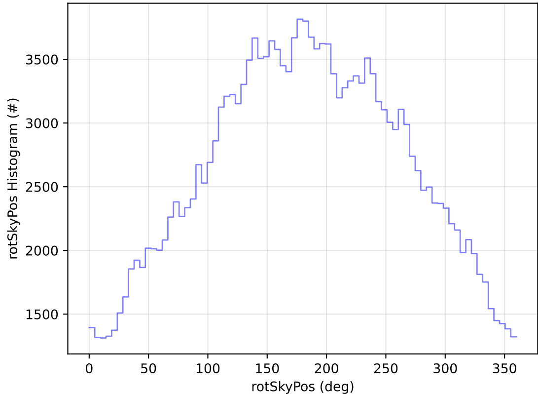
too_elab_2yr_r64_d3_ugrizy_v3.4_10yrs All sky g band: rotSkyPos Histogram
