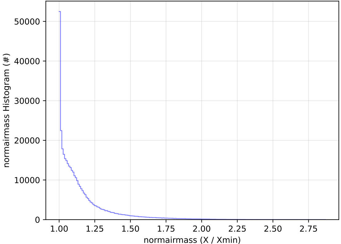
too_elab_2yr_r64_d3_ugrizy_v3.4_10yrs WFD y band: normairmass Histogram
