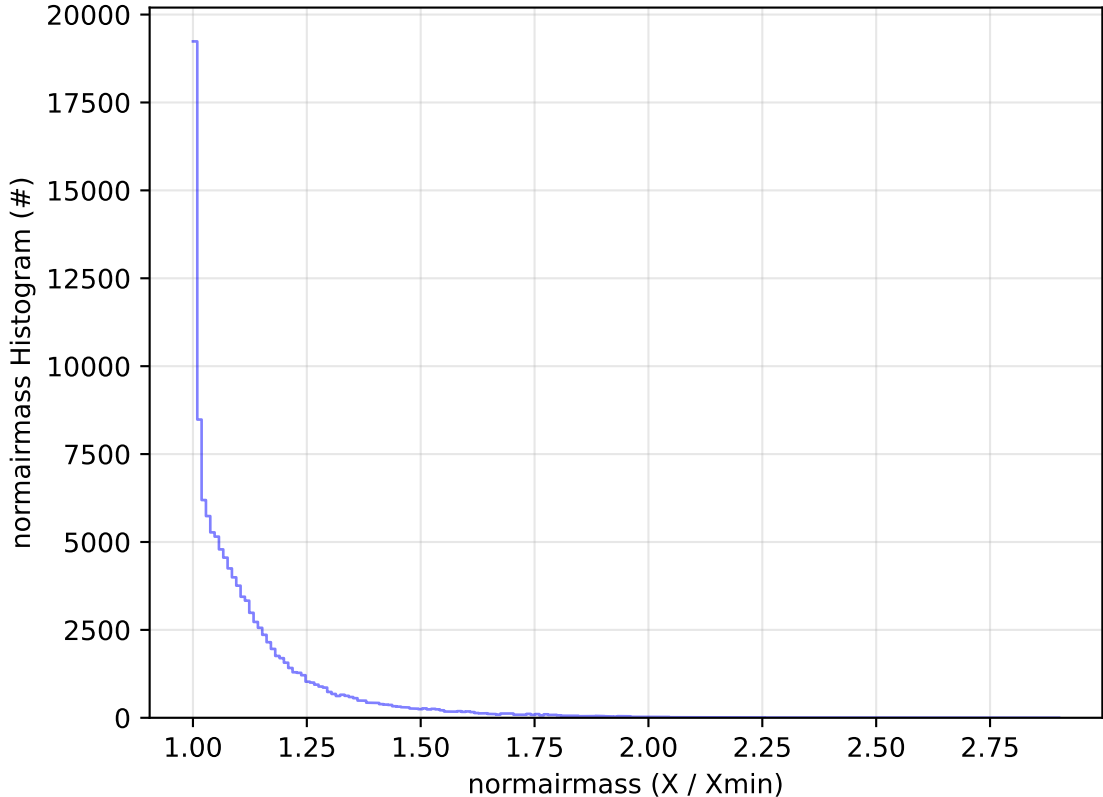
too_elab_2yr_r64_d3_ugrizy_v3.4_10yrs WFD u band: normairmass Histogram
