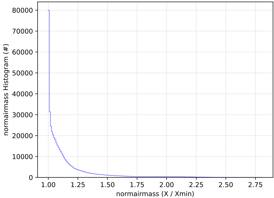
too_elab_2yr_r64_d3_ugrizy_v3.4_10yrs WFD r band: normairmass Histogram
