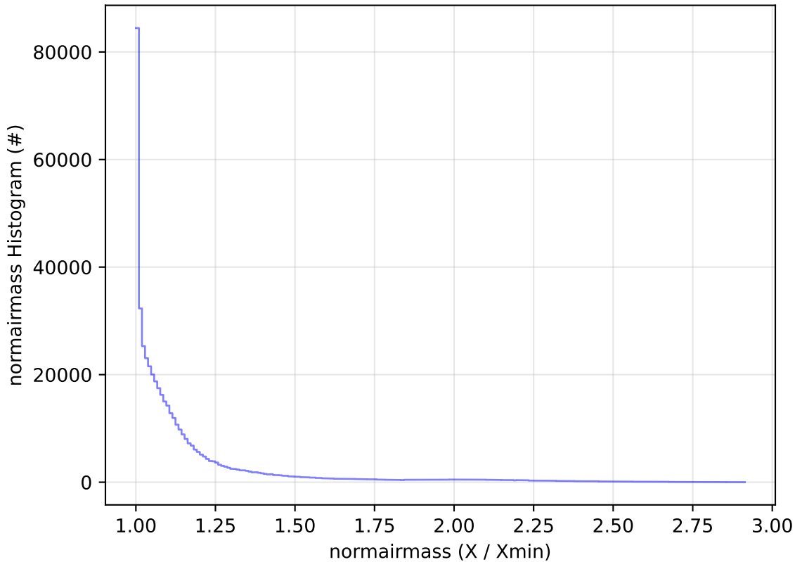
too_elab_2yr_r64_d3_ugrizy_v3.4_10yrs WFD i band: normairmass Histogram
