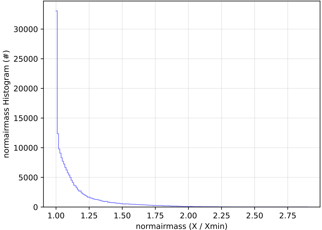
too_elab_2yr_r64_d3_ugrizy_v3.4_10yrs WFD g band: normairmass Histogram
