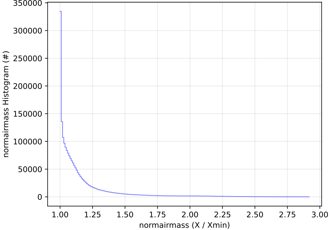
too_elab_2yr_r64_d3_ugrizy_v3.4_10yrs WFD all bands: normairmass Histogram
