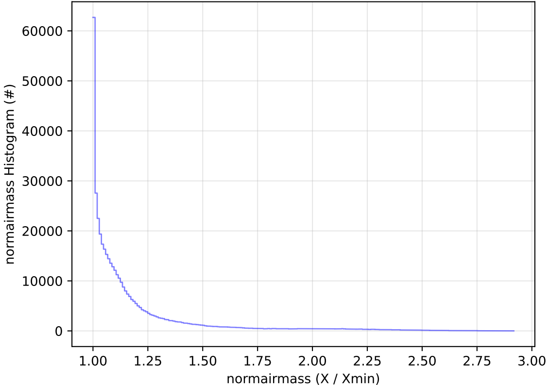
too_elab_2yr_r64_d3_ugrizy_v3.4_10yrs All sky z band: normairmass Histogram
