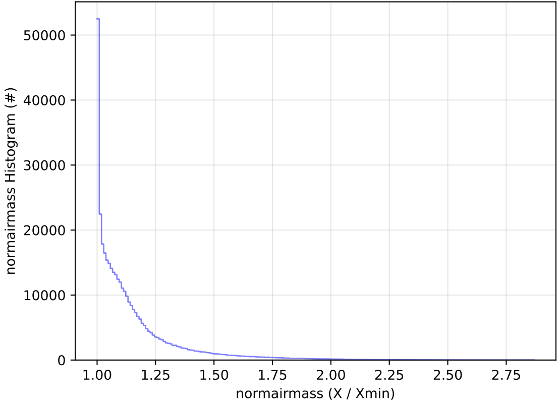
too_elab_2yr_r64_d3_ugrizy_v3.4_10yrs All sky y band: normairmass Histogram
