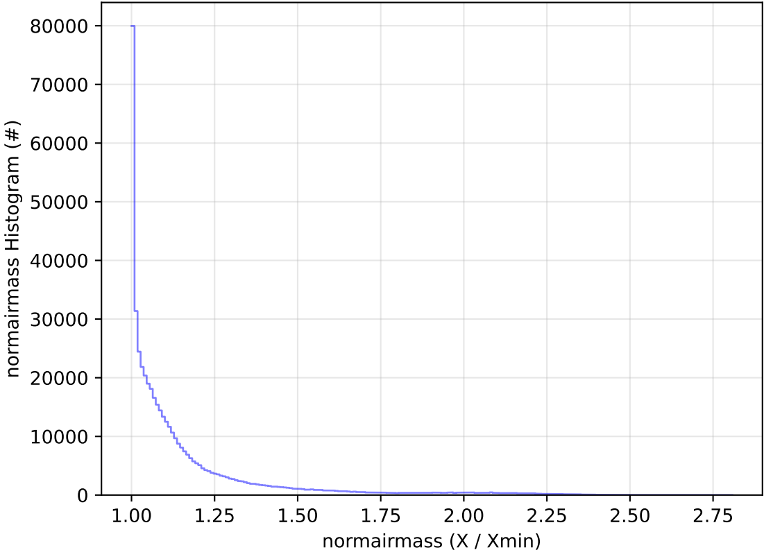
too_elab_2yr_r64_d3_ugrizy_v3.4_10yrs All sky r band: normairmass Histogram
