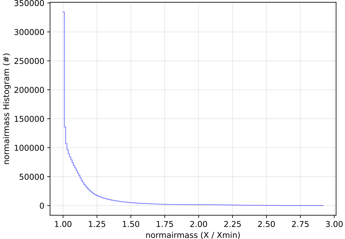
too_elab_2yr_r64_d3_ugrizy_v3.4_10yrs All sky all bands: normairmass Histogram
