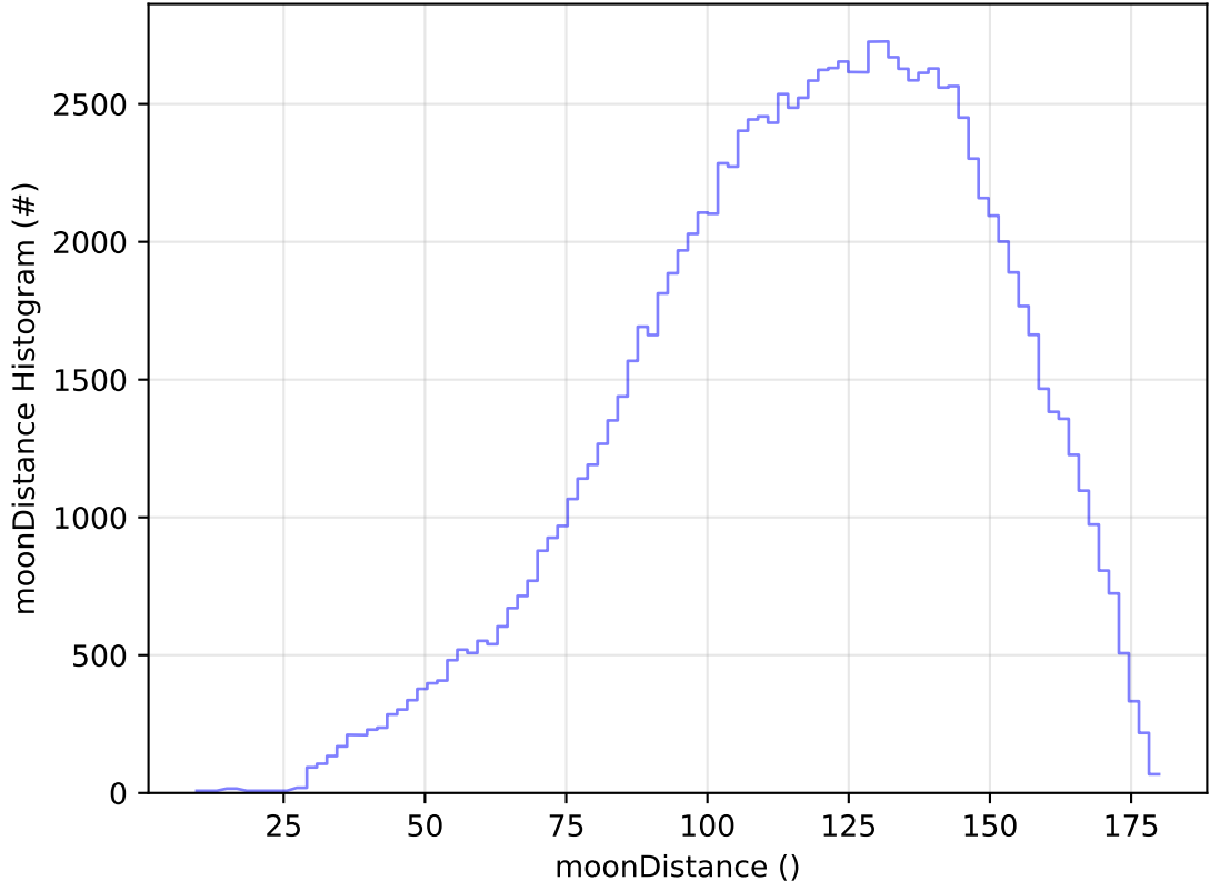
too_elab_2yr_r64_d3_ugrizy_v3.4_10yrs WFD u band: moonDistance Histogram
