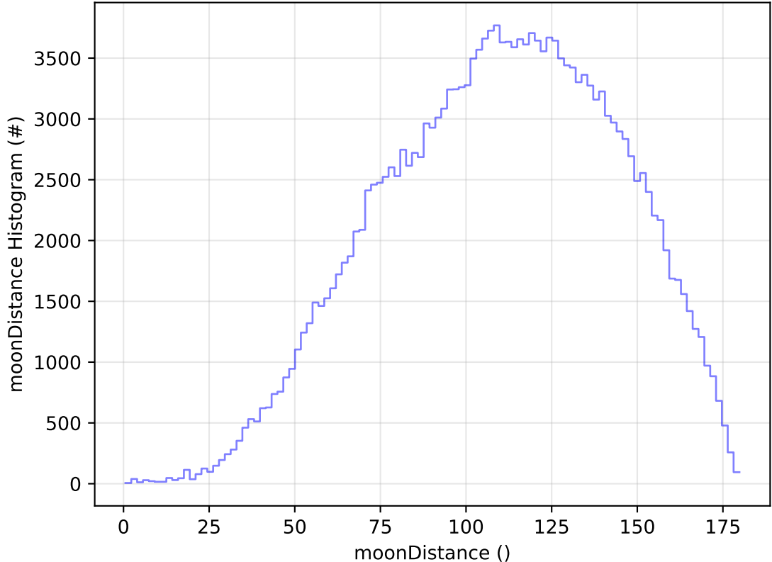
too_elab_2yr_r64_d3_ugrizy_v3.4_10yrs WFD g band: moonDistance Histogram
