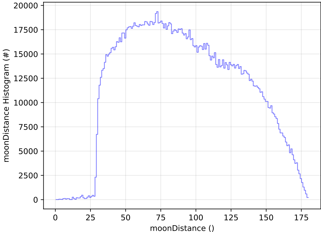
too_elab_2yr_r64_d3_ugrizy_v3.4_10yrs WFD all bands: moonDistance Histogram
