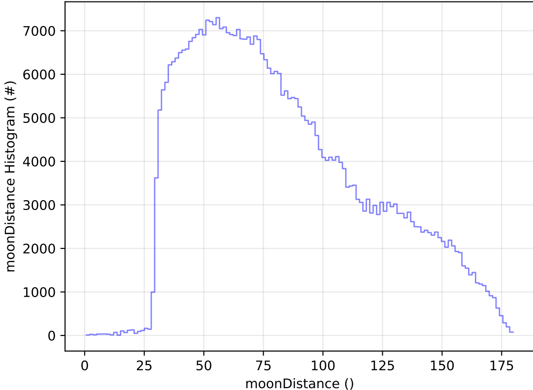
too_elab_2yr_r64_d3_ugrizy_v3.4_10yrs All sky z band: moonDistance Histogram
