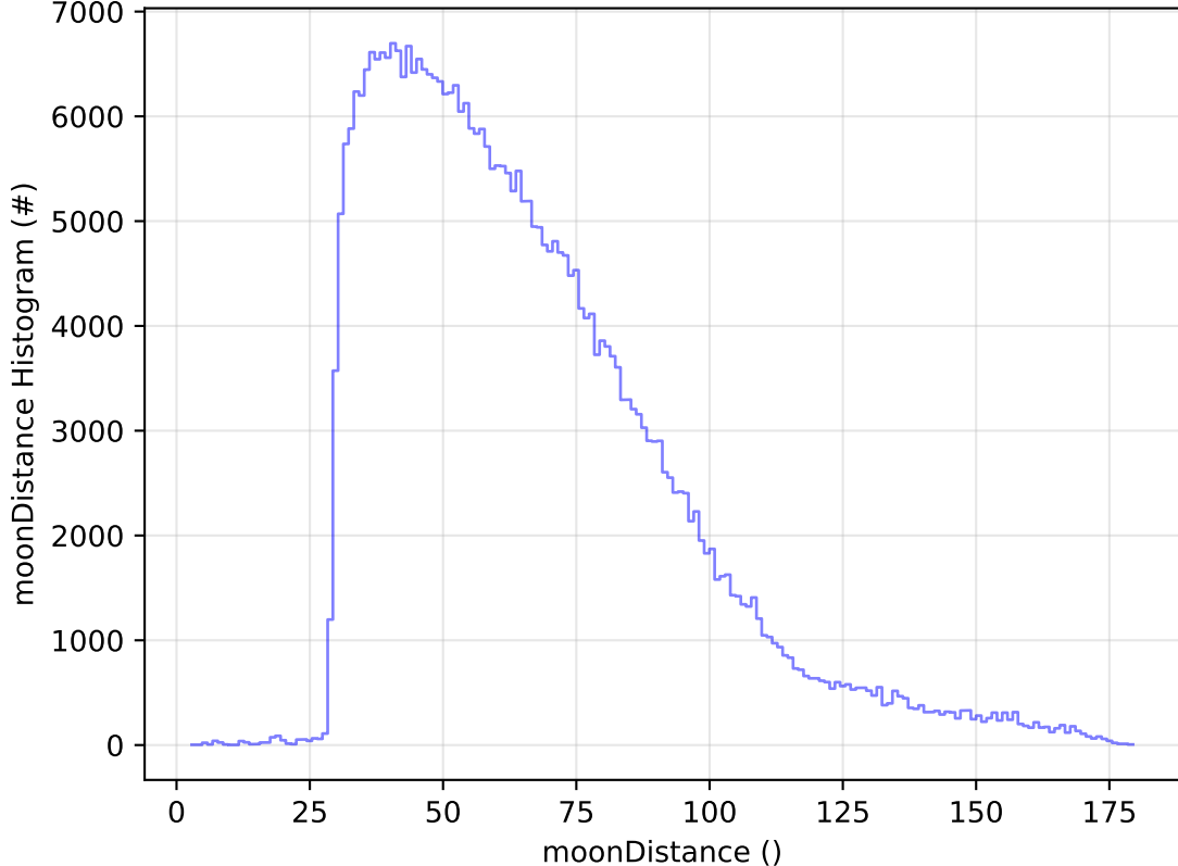
too_elab_2yr_r64_d3_ugrizy_v3.4_10yrs All sky y band: moonDistance Histogram
