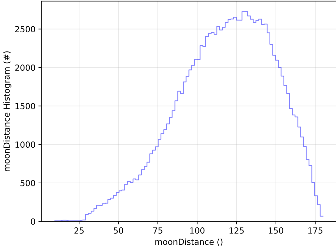
too_elab_2yr_r64_d3_ugrizy_v3.4_10yrs All sky u band: moonDistance Histogram
