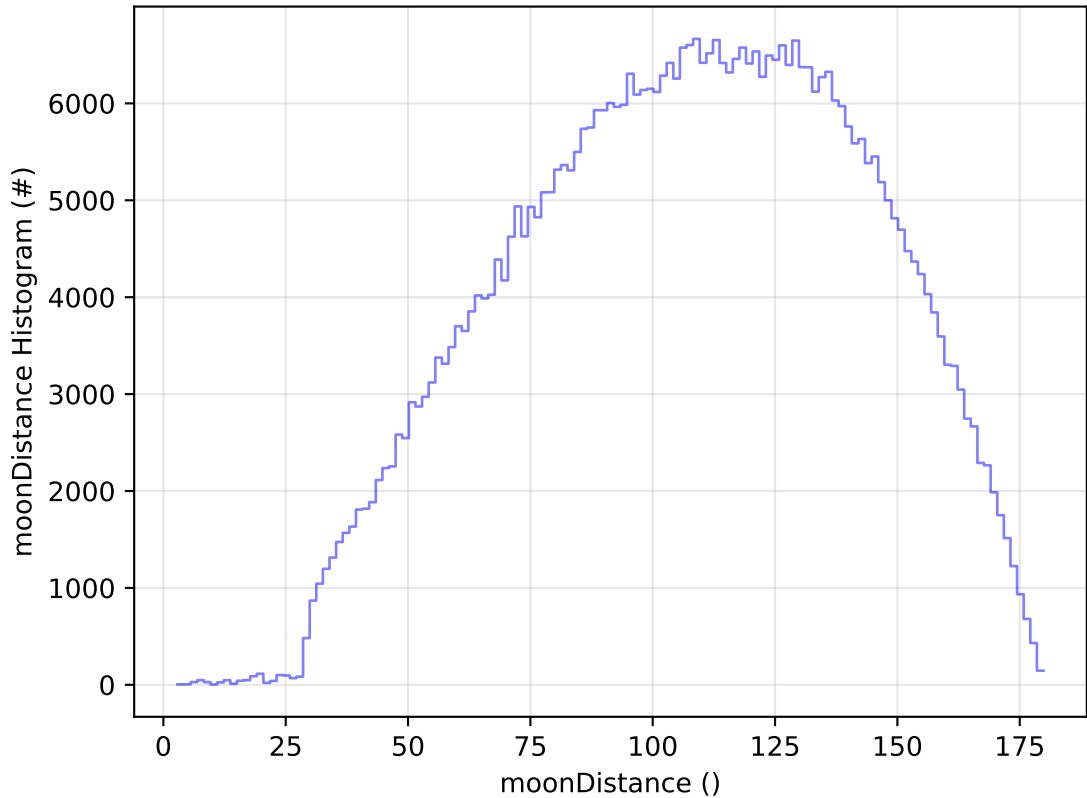
too_elab_2yr_r64_d3_ugrizy_v3.4_10yrs All sky r band: moonDistance Histogram
