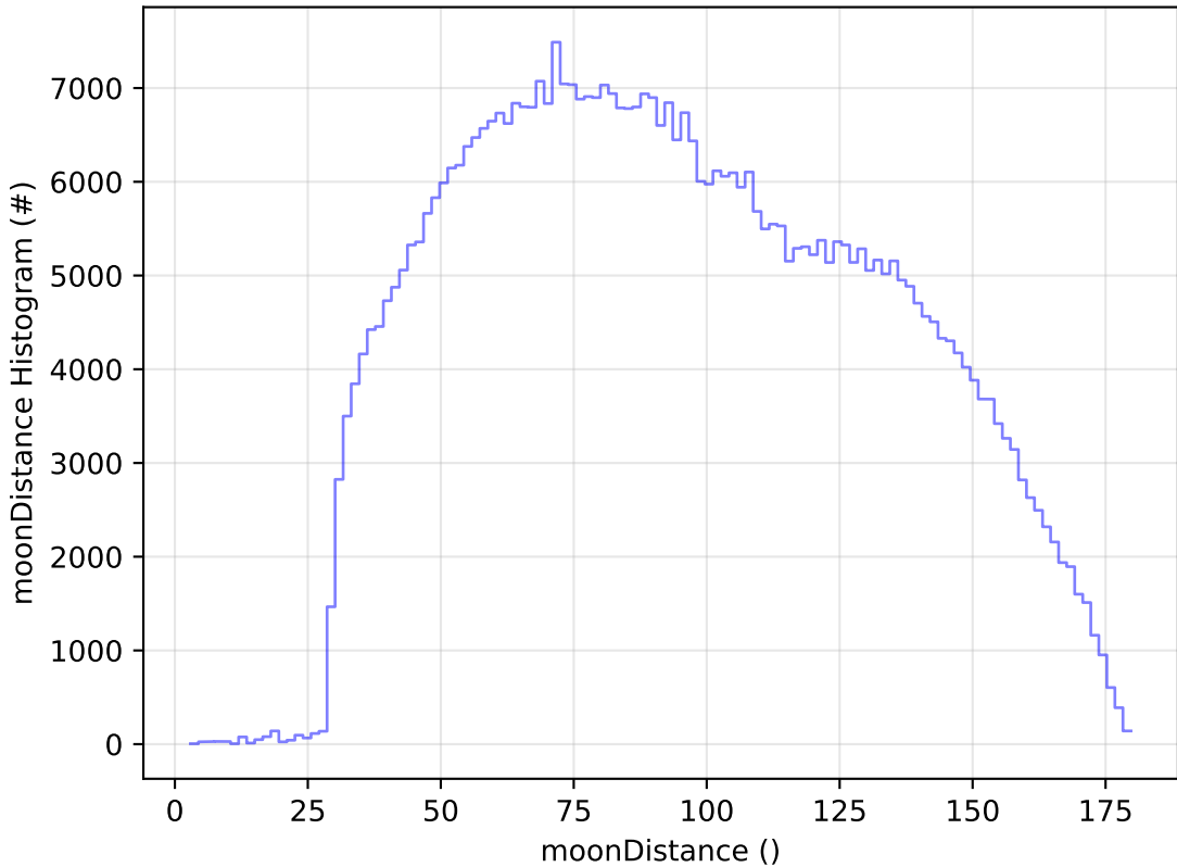
too_elab_2yr_r64_d3_ugrizy_v3.4_10yrs All sky i band: moonDistance Histogram
