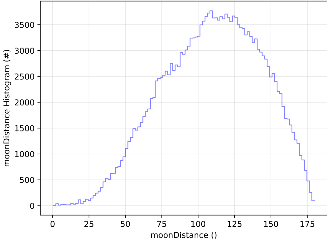
too_elab_2yr_r64_d3_ugrizy_v3.4_10yrs All sky g band: moonDistance Histogram
