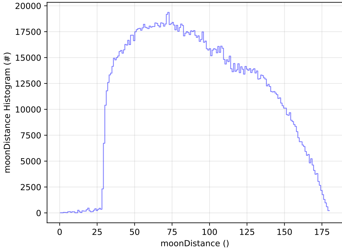
too_elab_2yr_r64_d3_ugrizy_v3.4_10yrs All sky all bands: moonDistance Histogram
