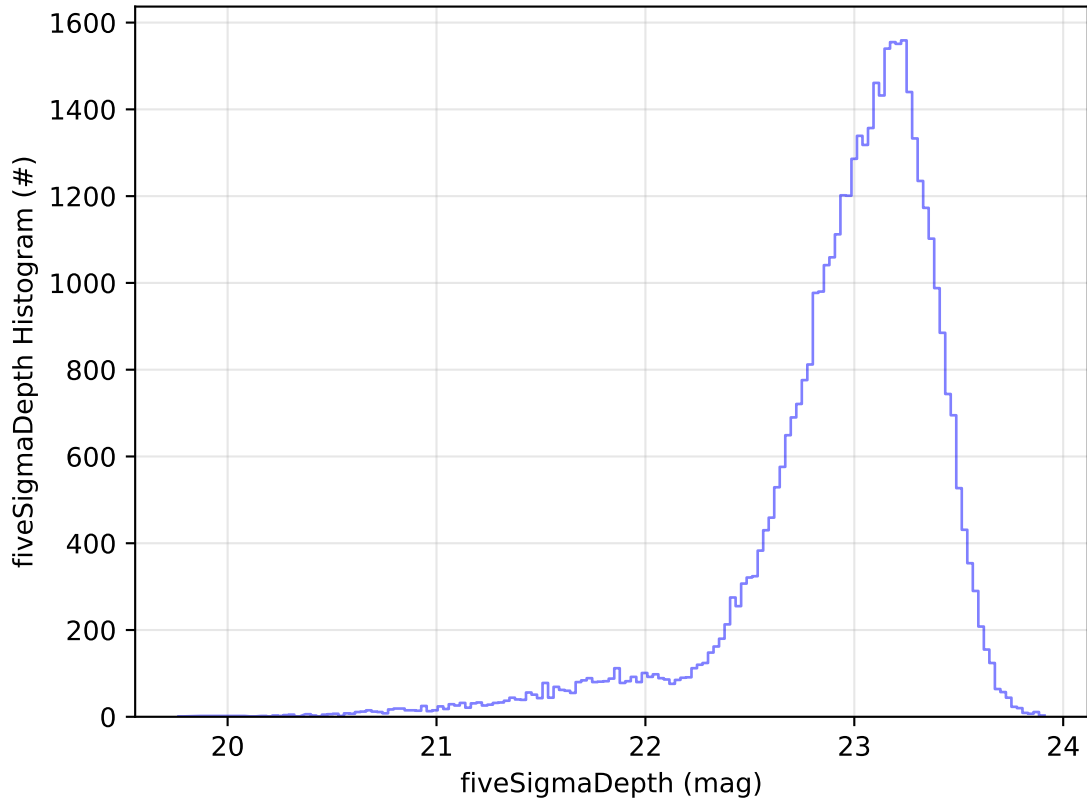
too_elab_2yr_r64_d3_ugrizy_v3.4_10yrs Yr 1 z band: fiveSigmaDepth Histogram
