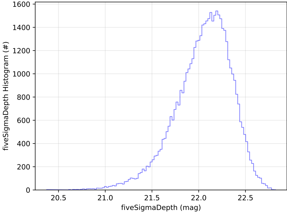
too_elab_2yr_r64_d3_ugrizy_v3.4_10yrs Yr 1 y band: fiveSigmaDepth Histogram
