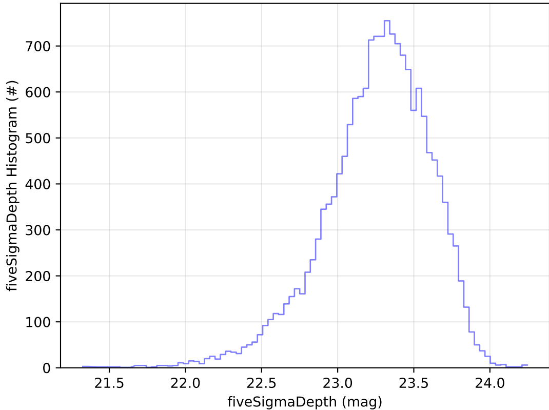
too_elab_2yr_r64_d3_ugrizy_v3.4_10yrs Yr 1 u band: fiveSigmaDepth Histogram
