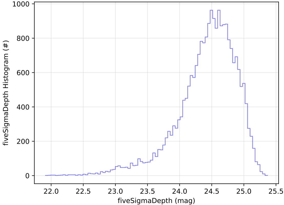
too_elab_2yr_r64_d3_ugrizy_v3.4_10yrs Yr 1 g band: fiveSigmaDepth Histogram
