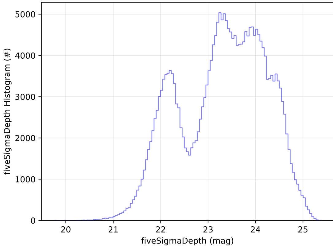
too_elab_2yr_r64_d3_ugrizy_v3.4_10yrs Yr 1 all bands: fiveSigmaDepth Histogram
