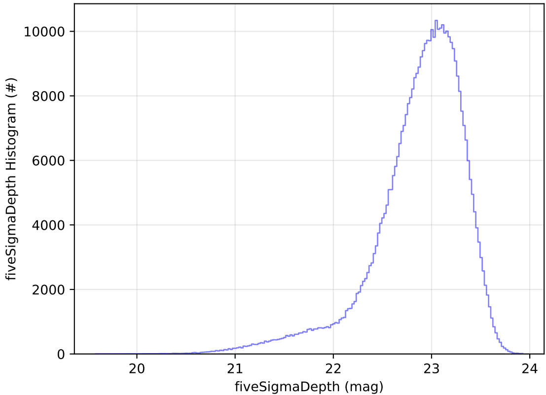
too_elab_2yr_r64_d3_ugrizy_v3.4_10yrs WFD z band: fiveSigmaDepth Histogram
