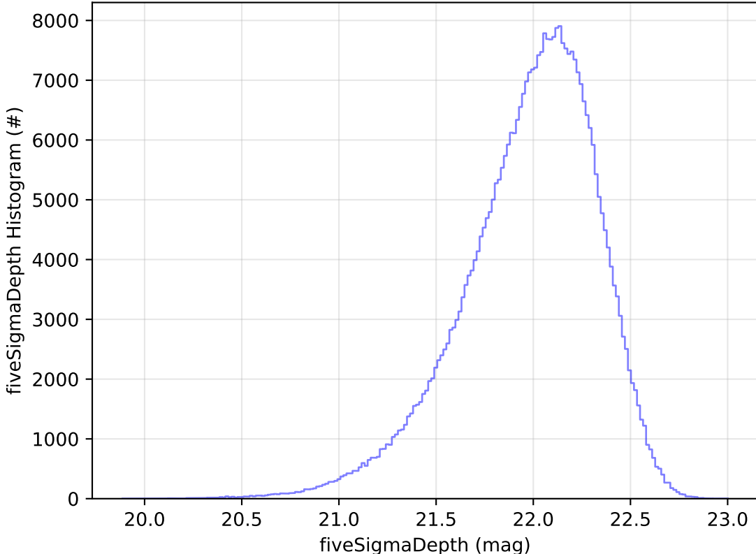
too_elab_2yr_r64_d3_ugrizy_v3.4_10yrs WFD y band: fiveSigmaDepth Histogram
