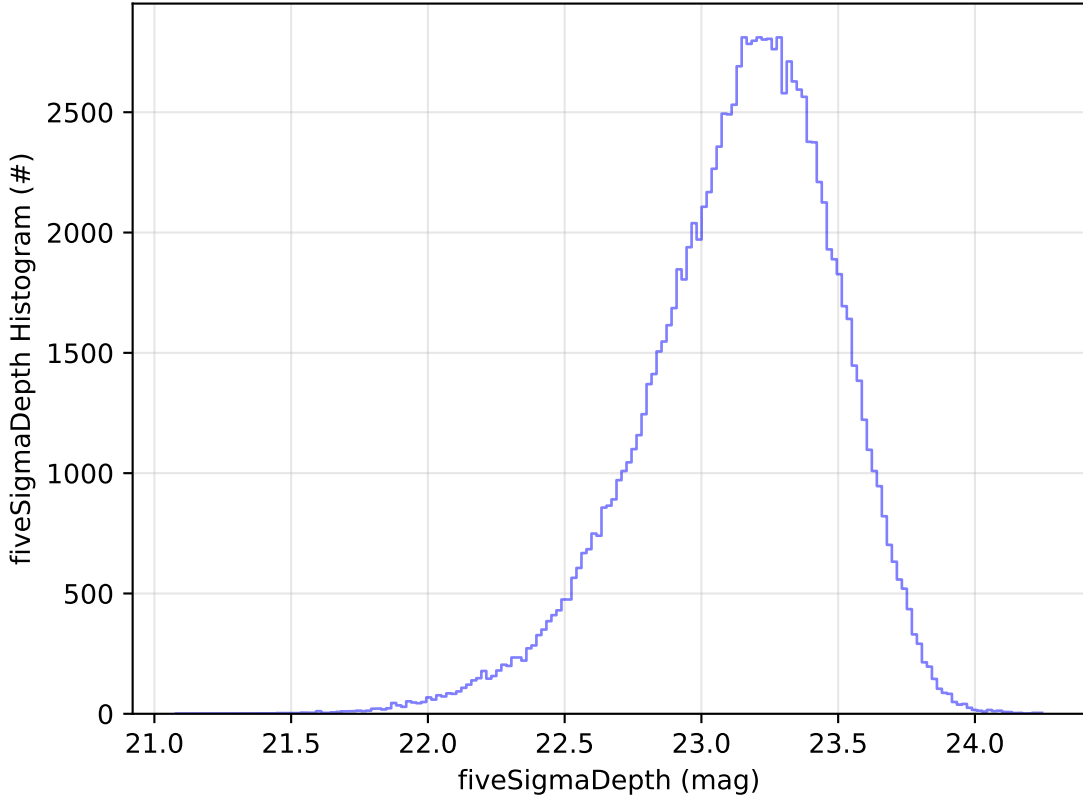
too_elab_2yr_r64_d3_ugrizy_v3.4_10yrs WFD u band: fiveSigmaDepth Histogram
