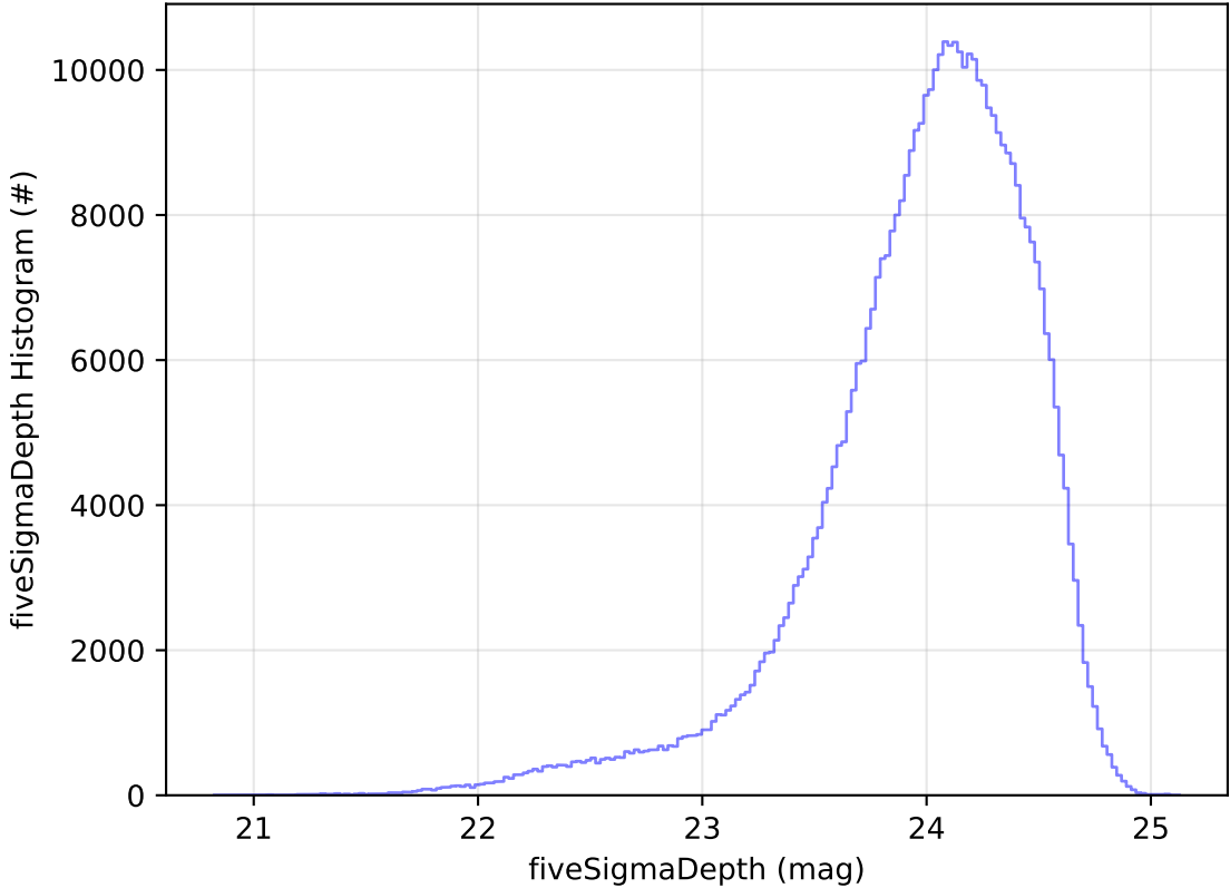
too_elab_2yr_r64_d3_ugrizy_v3.4_10yrs WFD r band: fiveSigmaDepth Histogram
