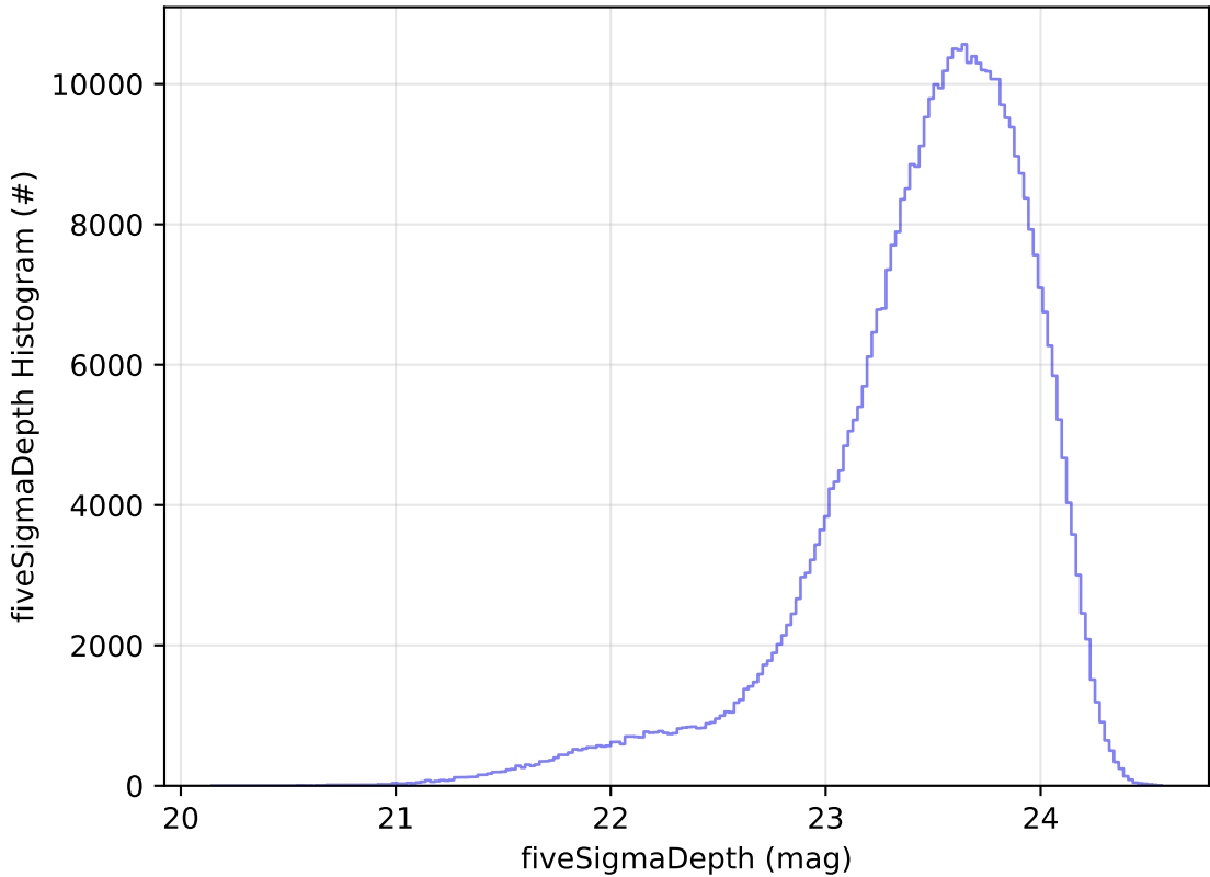
too_elab_2yr_r64_d3_ugrizy_v3.4_10yrs WFD i band: fiveSigmaDepth Histogram
