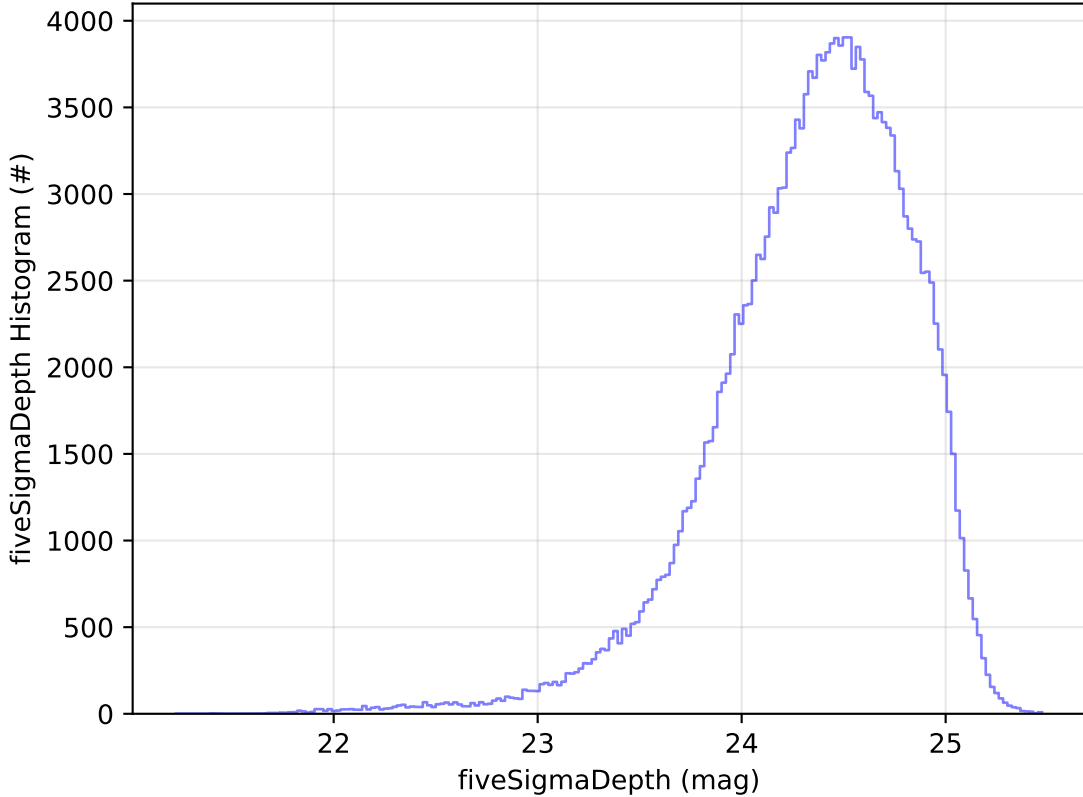
too_elab_2yr_r64_d3_ugrizy_v3.4_10yrs WFD g band: fiveSigmaDepth Histogram
