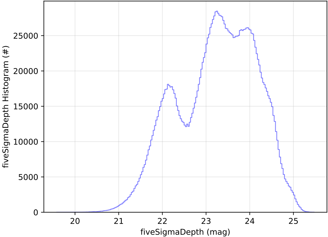
too_elab_2yr_r64_d3_ugrizy_v3.4_10yrs WFD all bands: fiveSigmaDepth Histogram
