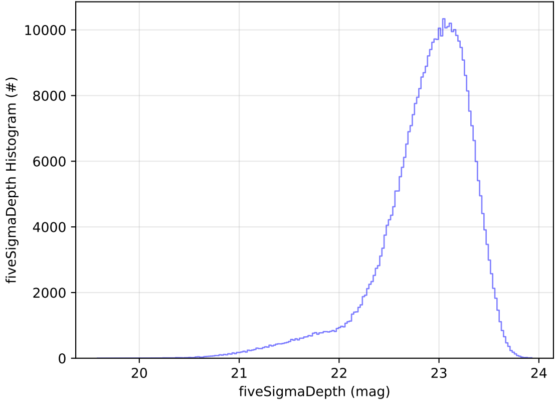
too_elab_2yr_r64_d3_ugrizy_v3.4_10yrs All sky z band: fiveSigmaDepth Histogram
