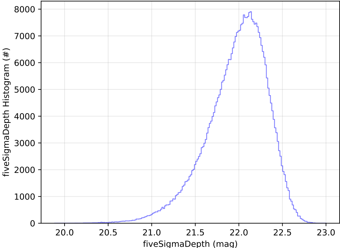
too_elab_2yr_r64_d3_ugrizy_v3.4_10yrs All sky y band: fiveSigmaDepth Histogram
