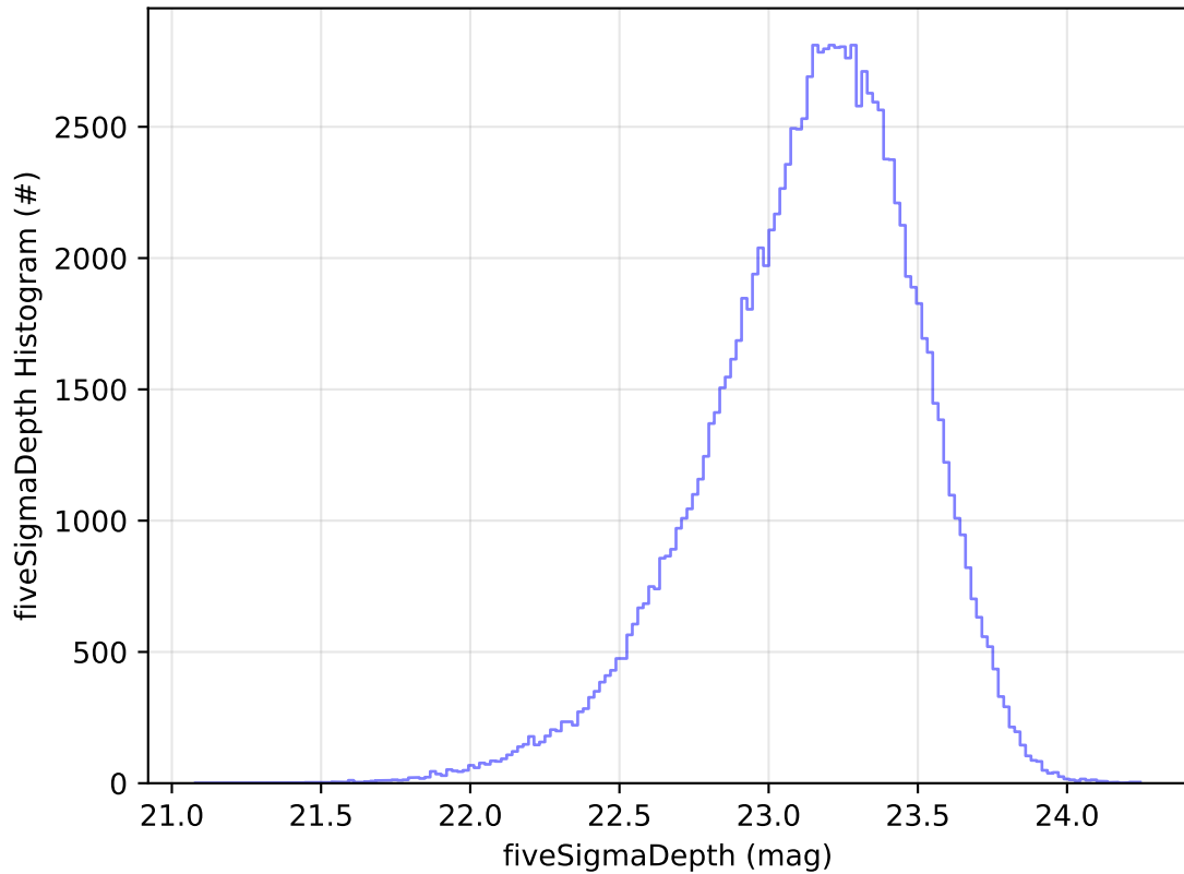
too_elab_2yr_r64_d3_ugrizy_v3.4_10yrs All sky u band: fiveSigmaDepth Histogram
