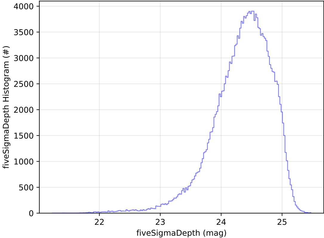
too_elab_2yr_r64_d3_ugrizy_v3.4_10yrs All sky g band: fiveSigmaDepth Histogram
