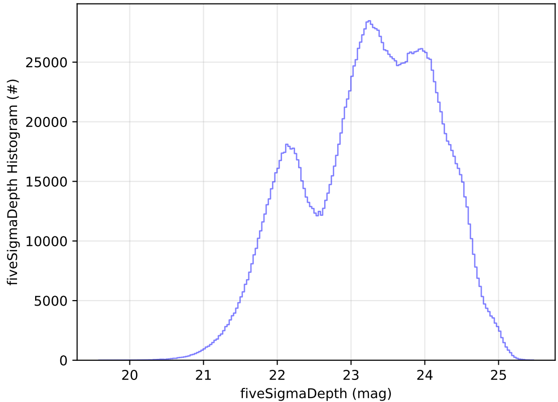
too_elab_2yr_r64_d3_ugrizy_v3.4_10yrs All sky all bands: fiveSigmaDepth Histogram
