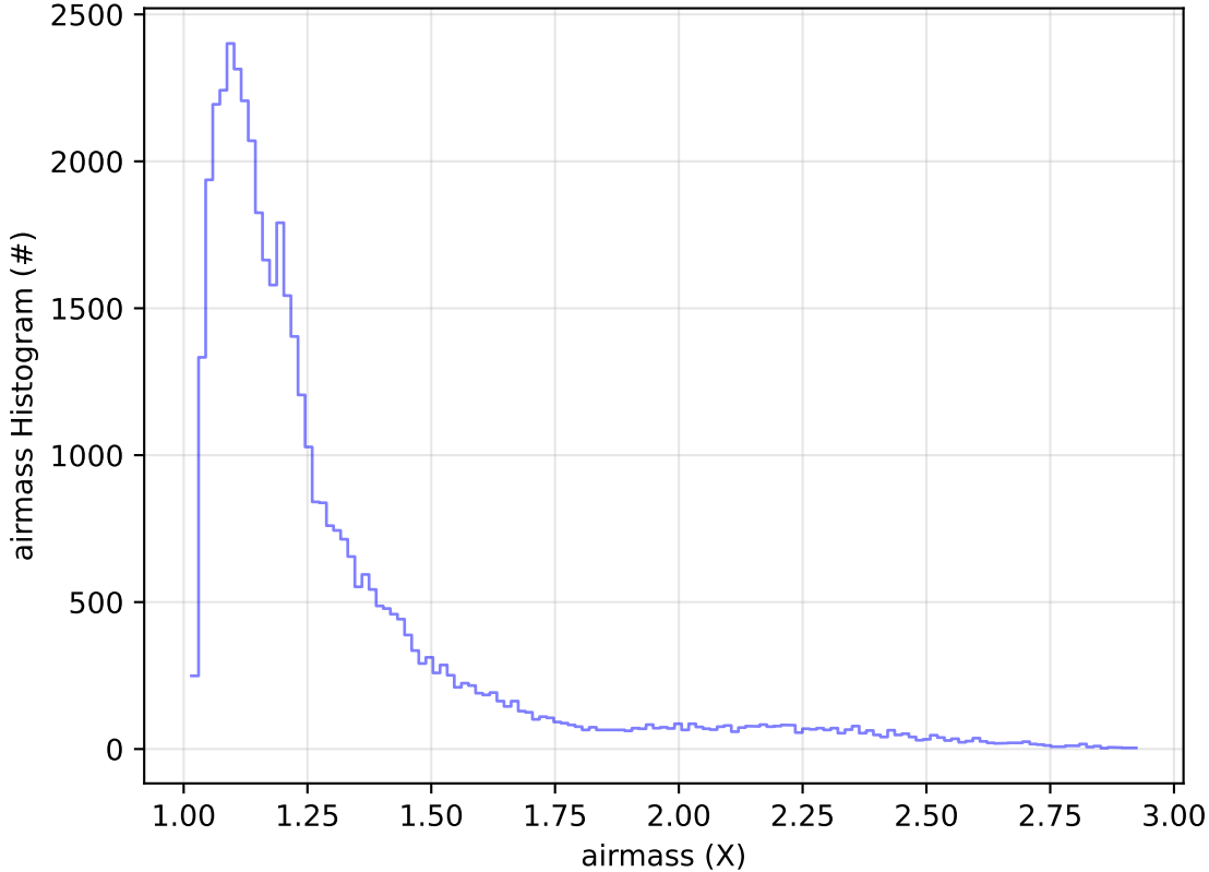
too_elab_2yr_r64_d3_ugrizy_v3.4_10yrs Yr 1 z band: airmass Histogram
