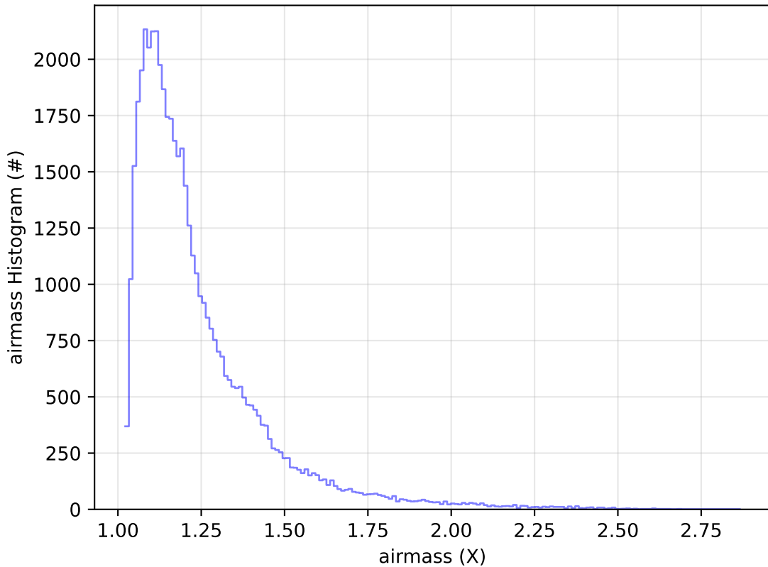
too_elab_2yr_r64_d3_ugrizy_v3.4_10yrs Yr 1 y band: airmass Histogram
