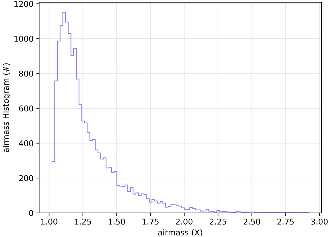
too_elab_2yr_r64_d3_ugrizy_v3.4_10yrs Yr 1 u band: airmass Histogram
